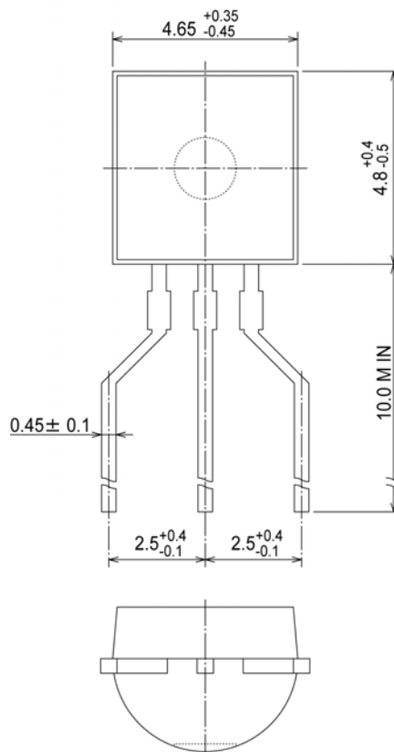
TO-92
